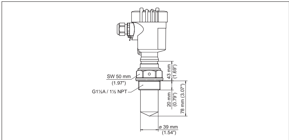
Fig. 63: VEGAPULS 61, rosca G1½, 1½ NPT
