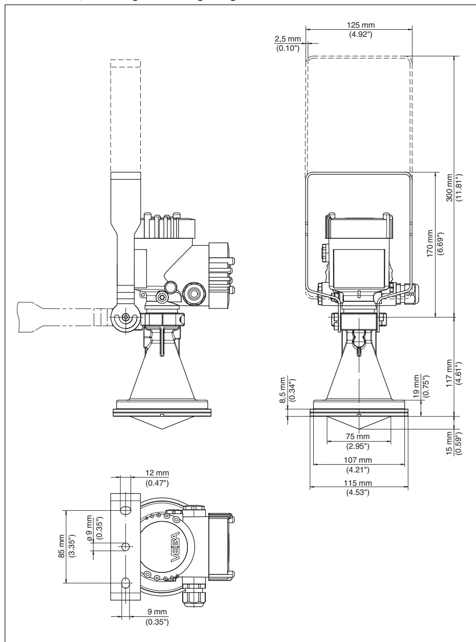
Fig. 57: VEGAPULS 61, montagebeugel in 170 of 300 mm lengte
