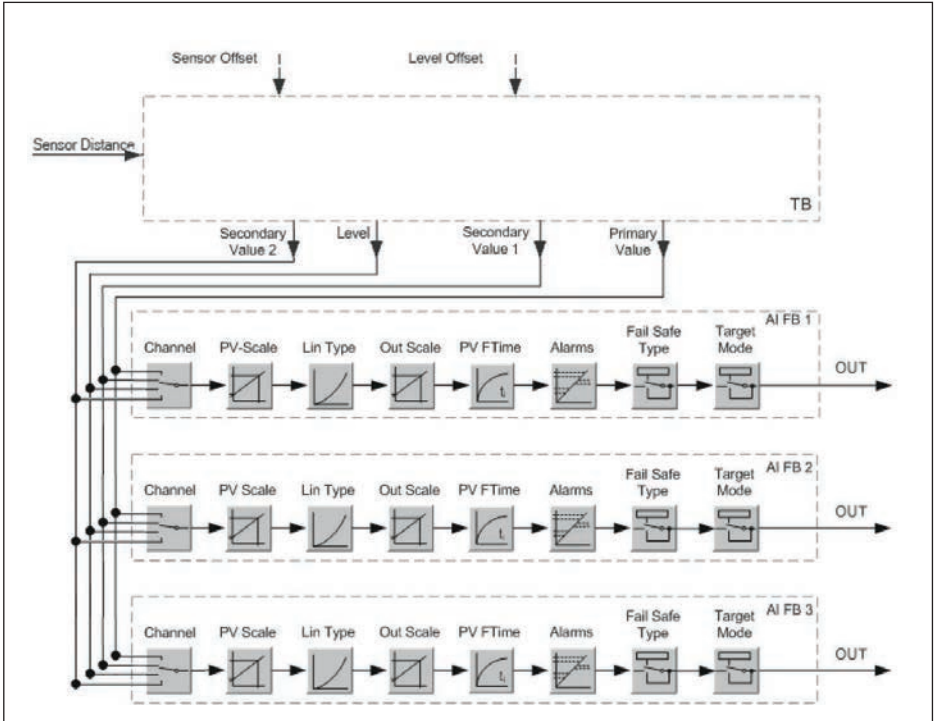
Res. 54: VEGAPULS 61: Block diagram with AI FB 1 ... AI FB 3 OUT values
