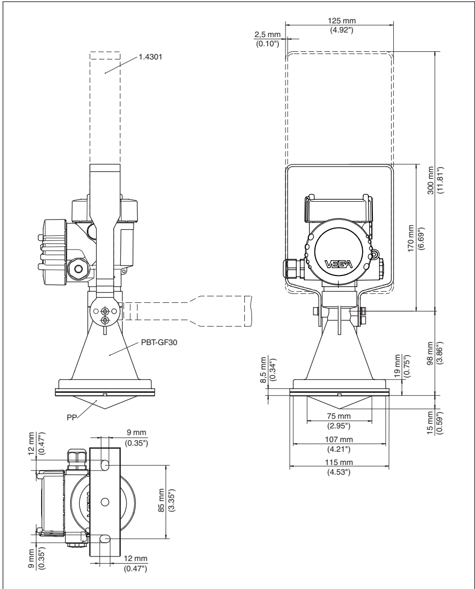
Fig. 57: VEGAPULS 61, montagebeugel in 170 of 300 mm lengte
