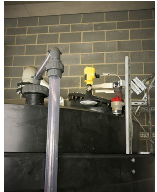
A VEGAPULS 64 radar sensor, mounted above a storage tank on a boom, measures the level of hydrochloric acid right through the top of the tank.
