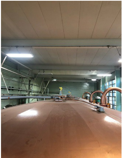
VEGAPULS 64 radar sensors with 80 GHz technology measure level in multiple fermenter vessels in the fermentation room.
