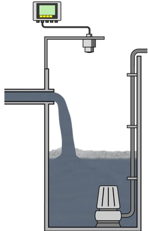
The very good signal focusing of VEGAPULS enables reliable detection of the product surface even in vessels with many internal installations.
