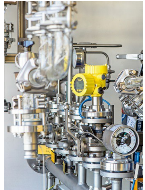
Ensuring simplified qualification: CARBOGEN AMCIS AG uses mostly identical, standardized pressure transmitters.
